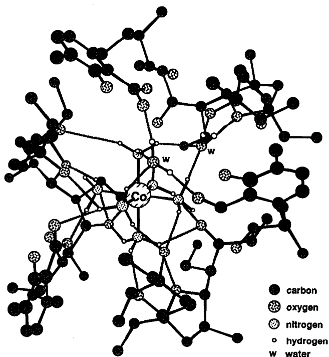
Fig. 6. The X-ray structure of the outersphere complex [\text{Co}(\text{NH}_3)_6] \cdot (\text{Las})_3 (Ref. [87]).
