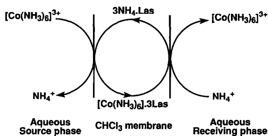
Fig. 7. Transport of [\text{Co}(\text{NH}_3)_6]^{3+} by lasalocid across a chloroform membrane coupled to an ammonium ion counter gradient.
