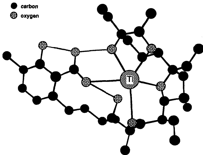
Fig. 4. The X-ray structure of the monomeric thallium complex of the lasalocid anion (Ref. [27]).
